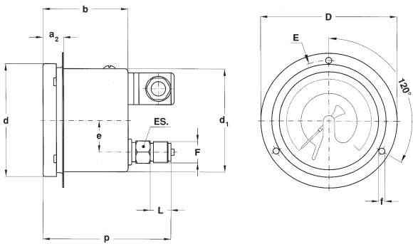
D + E flush mounting, front flange 3 holes; back connection.
