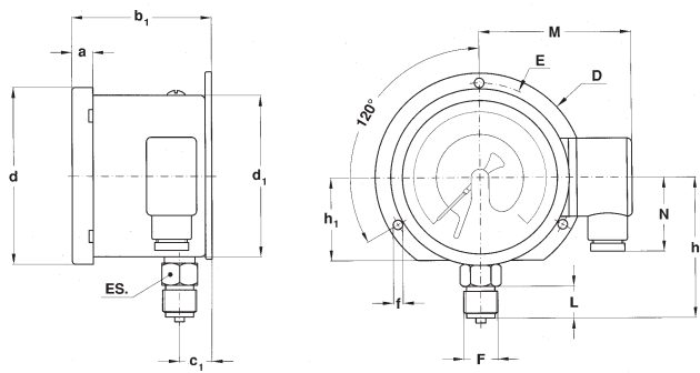
A + C surface mounting, back flange; lower connection.
