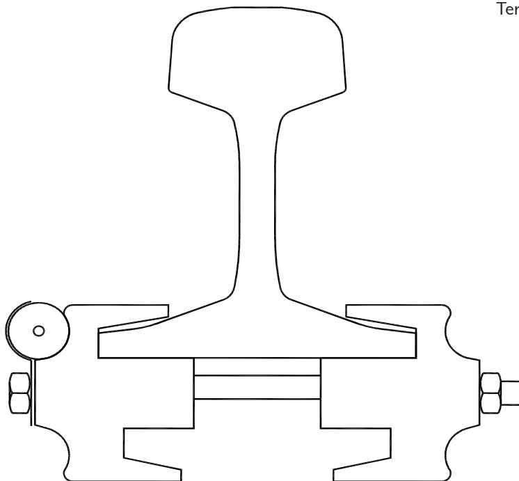
Rail attachment adapter part No.: 110404
