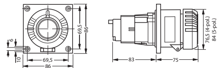
4/5-pole flange socket
