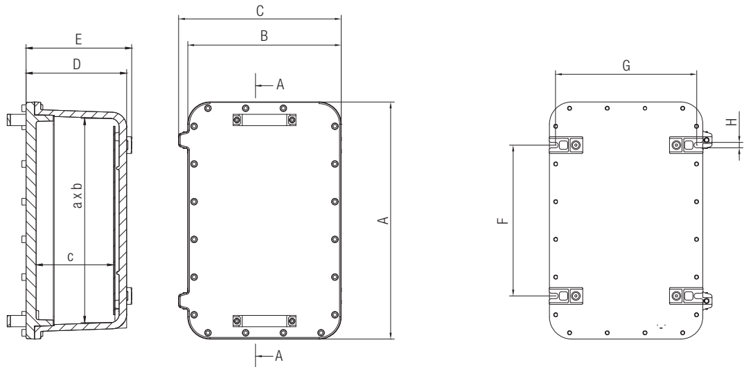
Overall dimensions and weights aluminium EJC
