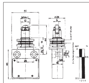
Front-mounting-roller lever 07-2951-..30/51
