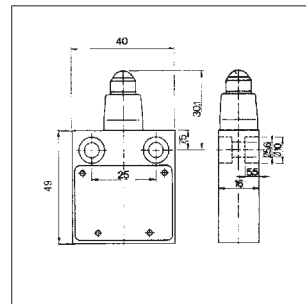
Membrane roller lever, long 07-2961-1.62/16
