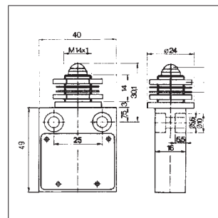
Front mounting/spherical plunger 07-2961-1.62/49
