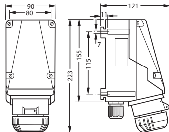
Dimensions 3-pole wall socket
