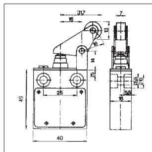
Parallel roller lever 07-2961-1.62/20
