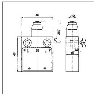
Membrane roller plunger 07-2961-1.62/10
