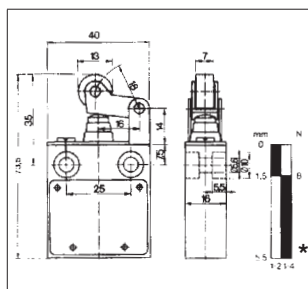
Feeler lever 07-2951-..30/32
