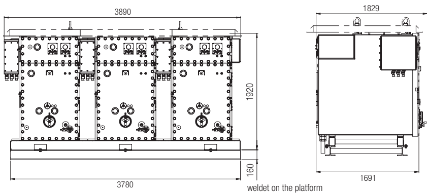
Dimensions Ring Main Unit
