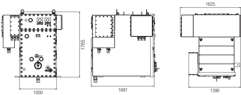
Dimensions Single Switchgear Vacuum Circuit Breaker
