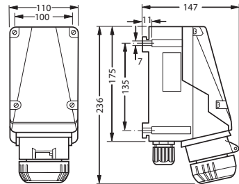
4/5-pole wall socket
