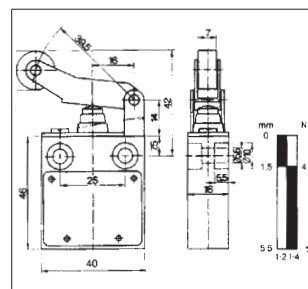
Feeler-butt lever 07-2951-..30/34
