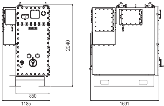
Dimensions Single Switchgear Vacuum Contactor
