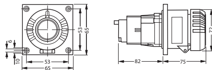
Dimensions 3-pole flange socket
