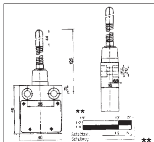
Feeler plastic lever 07-2951-..30/36
